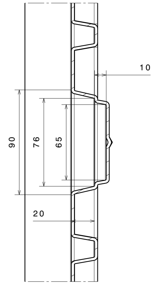
Section view D-D
